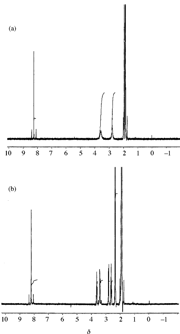
Fig. 3 The 500 MHz ^1\text{H} NMR spectra of [\text{Hg}(\text{imBT})]^{2+} at (a) 323 and (b) 240 K.
